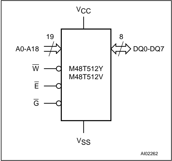
Figure 2. Logic Diagram
